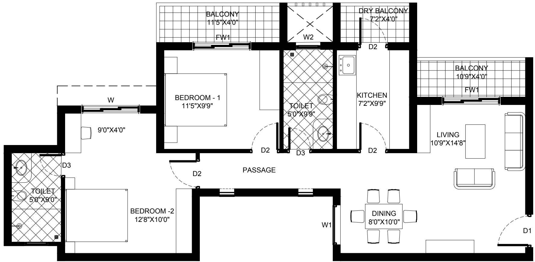
FLOOR PLAN (2-BHK)
